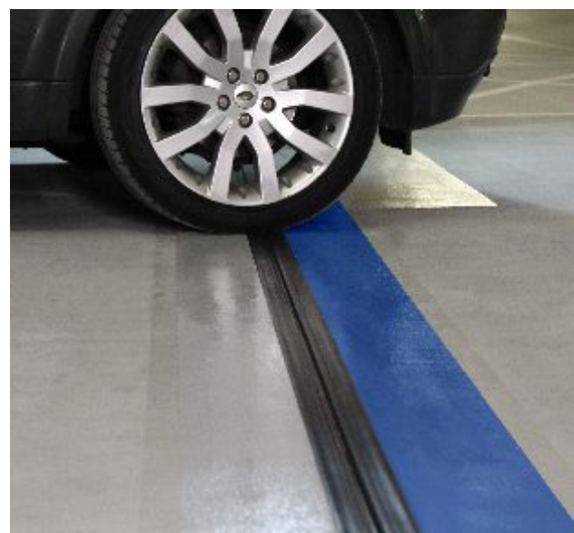
FloorBridge® CPS 20/50 DUO with one-sided coating connection
