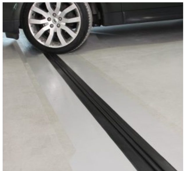
FloorBridge® CPS 20/80 DUO with one-sided coating connection
